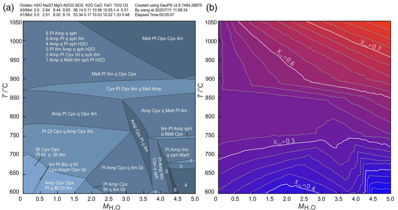
FIGURE 7 GeoPS calculated T - M_{H_2O} section of sample BL478 at 7 kbar (a) and an isopleth of X_{An} of plagioclase (b)
