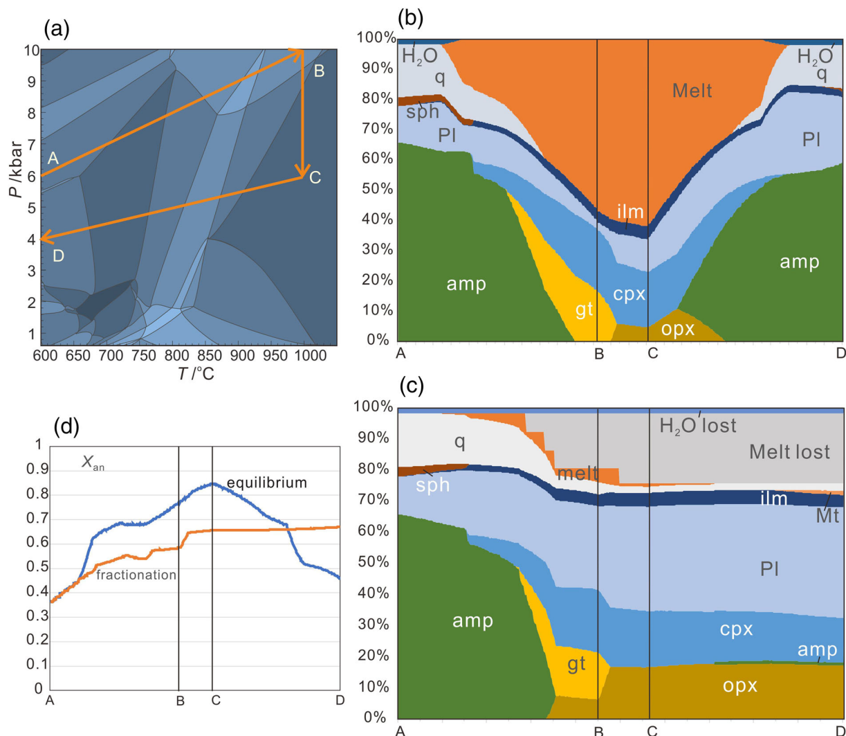
FIGURE 8 Phase equilibrium modelling for BL487 along a hypothetical clockwise P - T path. (a) the hypothetical clockwise P - T path; (b and c) phase proportions along the clockwise P - T path with equilibrium model (b) and fractionation model (c); (d) X_{an} of plagioclase along the clockwise P - T path
